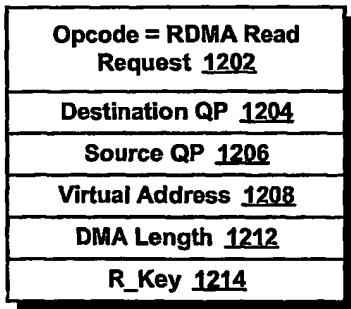
FIG. 12 (Related Art)
